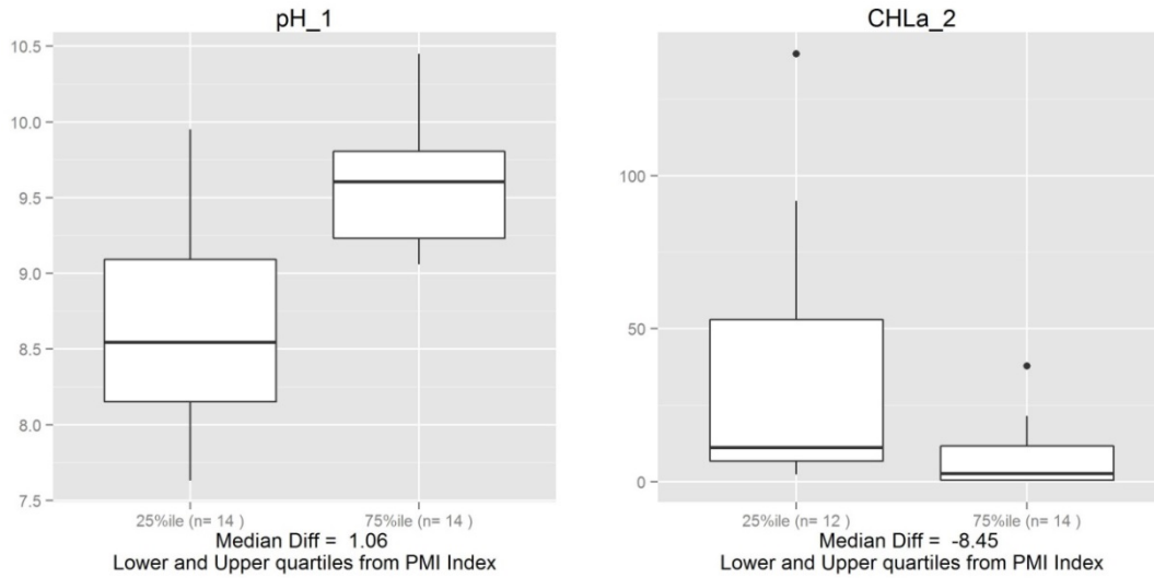
Figure A2-24. Response of macroinvertebrates to water column pH and chlorophyll a concentrations (units: unitless and µg/L).
