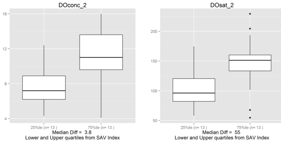
Figure A2-3. Response of SAV index to DO concentration and percentage saturation (units: mg/L and % saturation).
