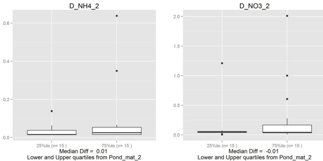
Figure A2-14. Response of surface mats to dissolved inorganic N concentrations (units: mg/L).
