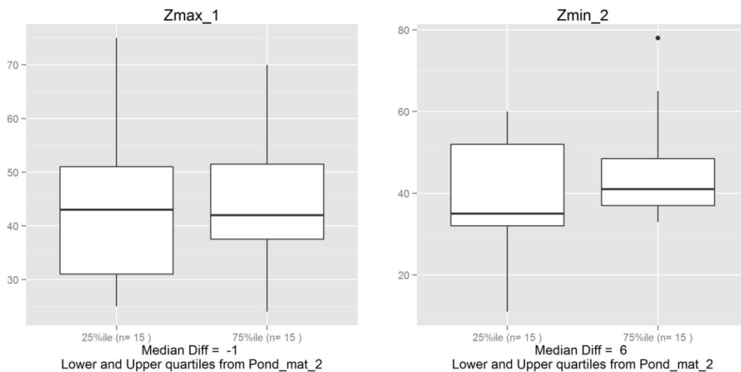
Figure A2-10. Response of surface mats to water depth (units: cm).
