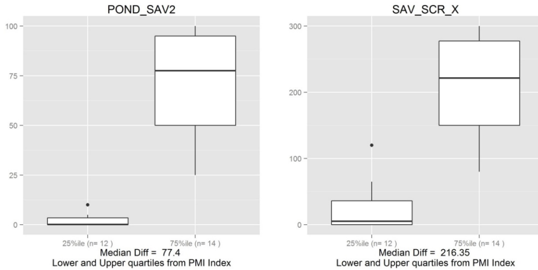
Figure A2-30. Response of macroinvertebrates to SAV cover and index scores (units: cover of pond surface and dimensionless index score).
