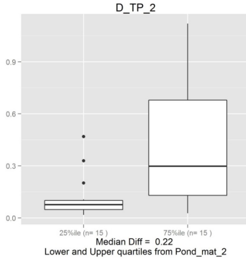
Figure A2-15. Response of surface mats to dissolved total phosphorus concentration (units: mg/L).
