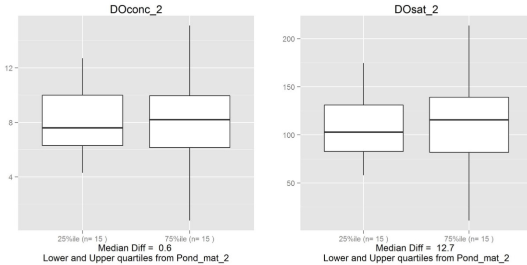
Figure A2-12. Response of surface mats to DO concentration (units: mg/L and % saturation).
