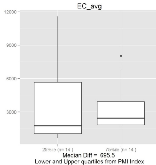
Figure A2-22. Response of macroinvertebrates to specific conductivity (units: uS/cm).
