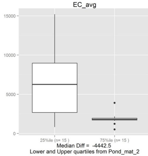
Figure A2-11. Response of surface mats to specific conductivity (units: uS/cm).
