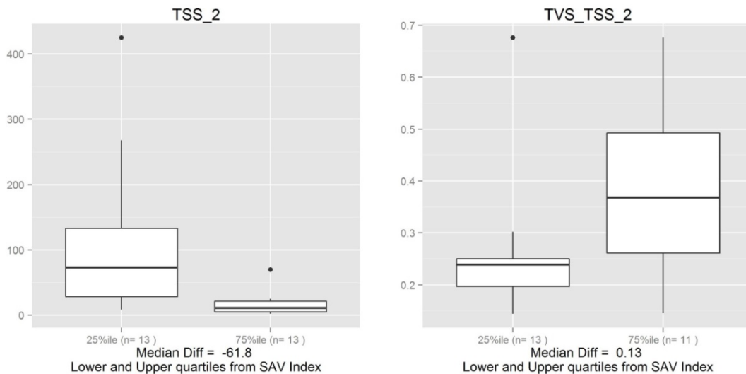
Figure A2-6. Response of SAV index to TSS and organic matter fraction of TSS (units: mg/L and mg organic matter/mg TSS).
