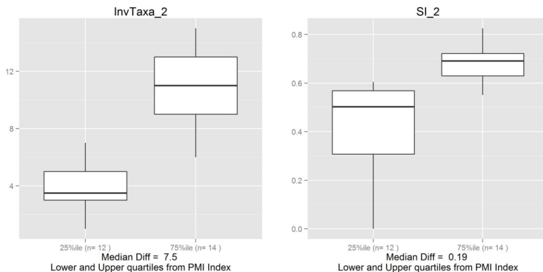
Figure A2-28. Response of macroinvertebrates to other invertebrate composition metrics (units: number of taxa and dimensionless index of community structure).
