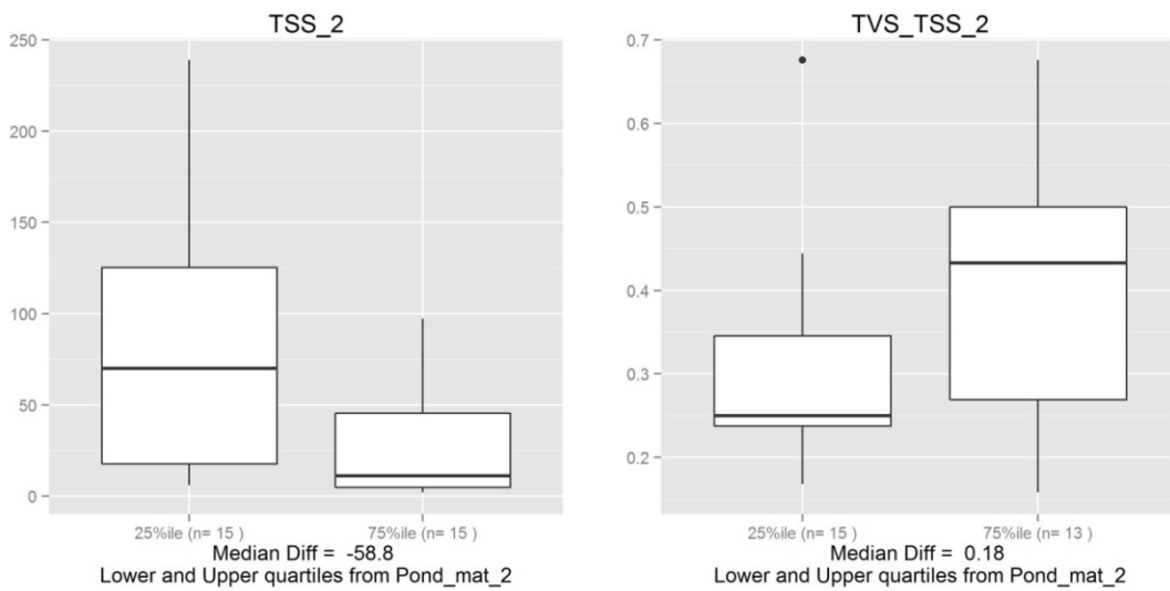
Figure A2-16. Response of surface mats to TSS and organic matter fraction of TSS (units: mg/L and mg OM/mg TSS).
