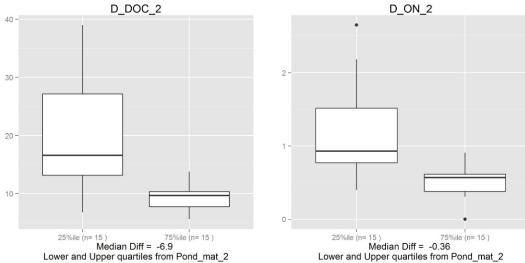
Figure A2-17. Response of surface mats to dissolved organic C and organic N concentrations (units mg/L).
