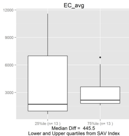
Figure A2-2. Response of SAV index to average specific conductivity (electrical conductivity, adjusted to 25°C; units: uS/cm).
