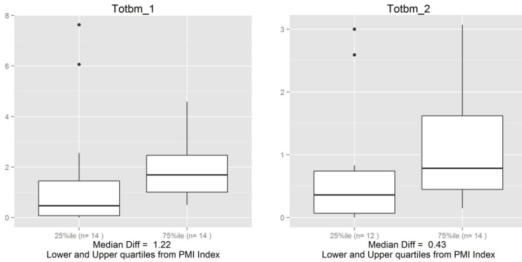
Figure A2-31. Response of macroinvertebrates to total invertebrate biomass (units: g/m 2 ).
