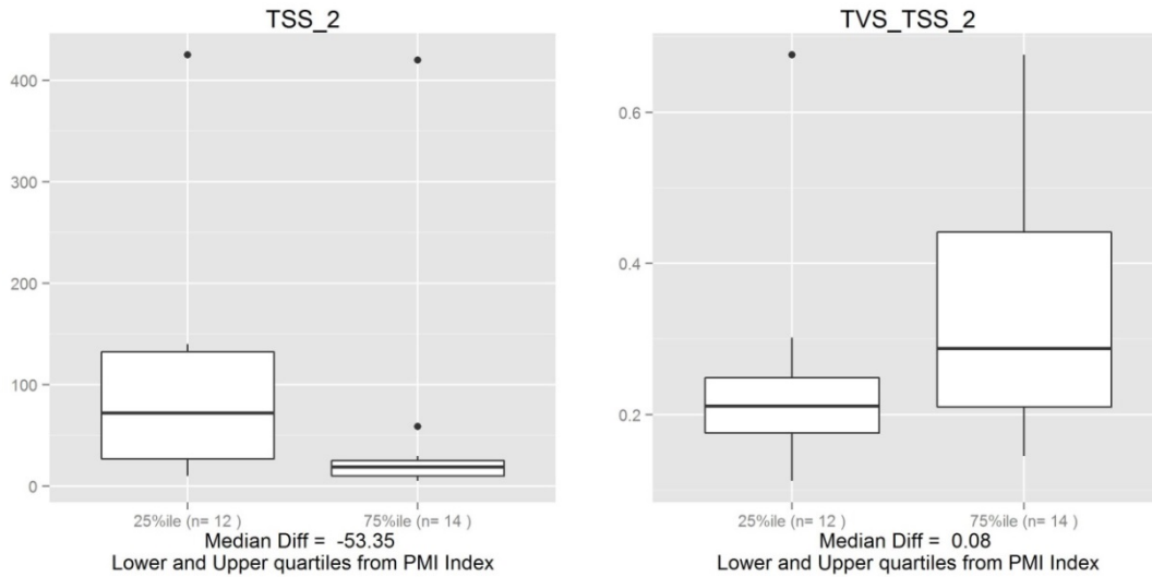
Figure A2-27. Response of macroinvertebrates to TSS and organic matter fraction of TSS (units: mg/L and mg OM/mg TSS).
