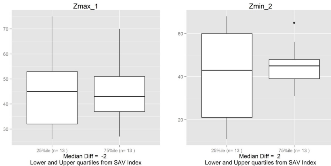
Figure A2-1. Response of SAV index to summer maximum water depth (left) and early autumn minimum water depth (right) (units: cm).
