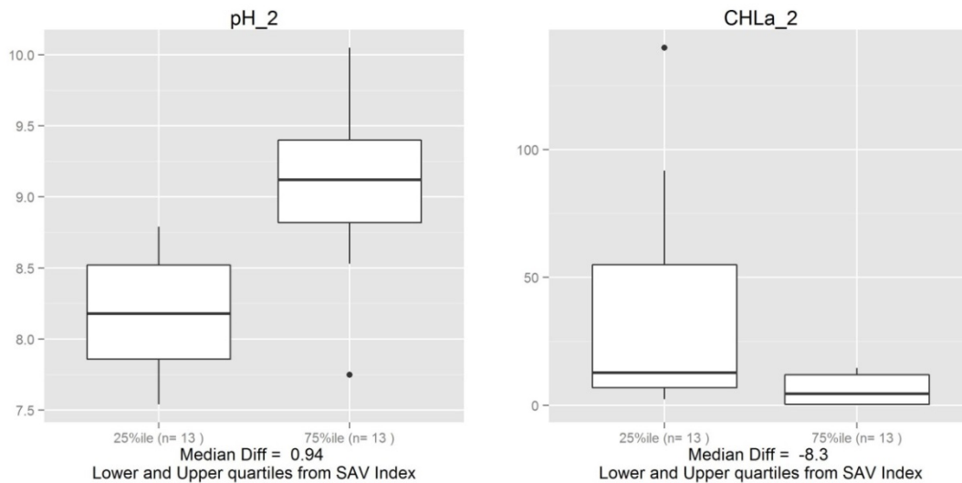
Figure A2-4. Response of SAV index to water column pH (field measure) and chlorophyll a concentrations (units: unitless and µg/L) .
