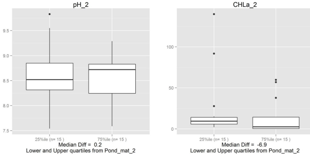
Figure A2-13. Response of surface mats to water column pH and chlorophyll a concentration (units: unitless and \mu\text{g/L} ).
