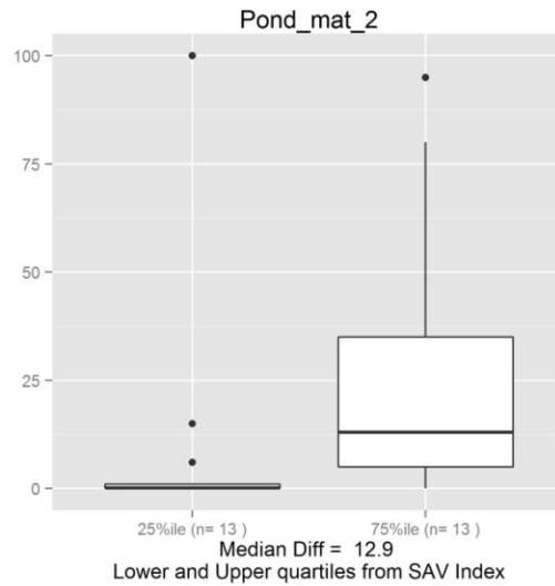
Figure A2-9. Response of SAV index to early autumn cover of surface mats (units: total cover of pond surface).
