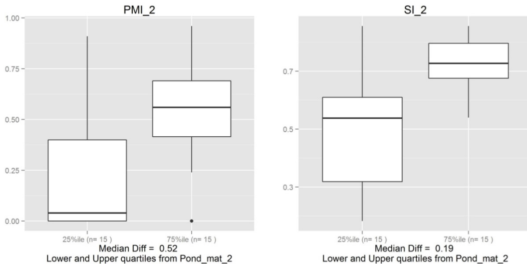
Figure A2-18. Response of surface mats to early autumn indices of macroinvertebrate communities (units: fraction of total invertebrate counts as PMI taxa, and dimensionless index of community structure).
