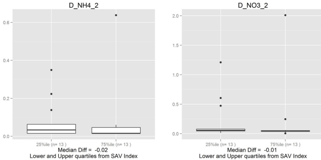
Figure A2-5. Response of SAV index to dissolved inorganic N concentrations (units: mg/L).
