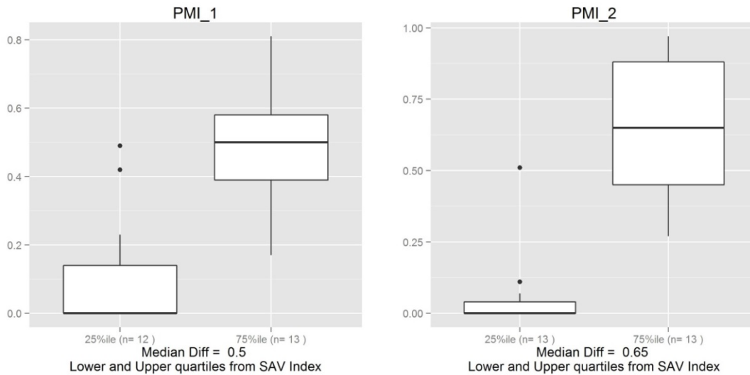
Figure A2-7. Response of SAV index to PMI index for macroinvertebrates (units: proportion of total sample count represented by PMI taxa).
