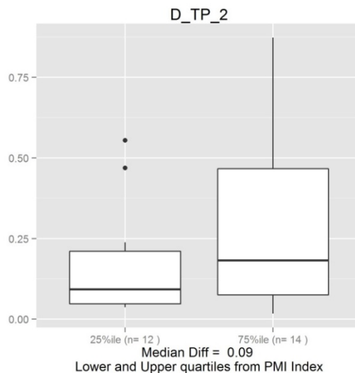
Figure A2-26. Response of macroinvertebrates to dissolved total phosphorus concentrations (units: mg/L).
