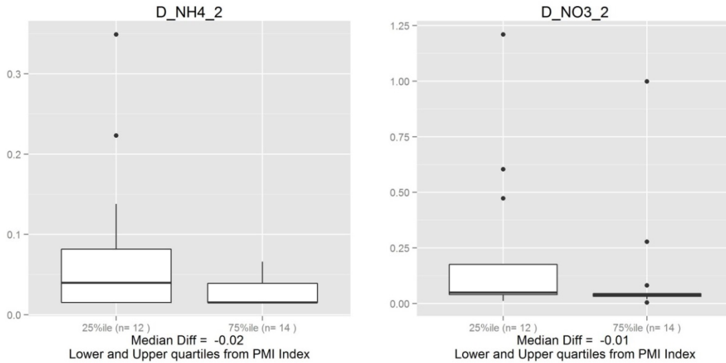
Figure A2-25. Response of macroinvertebrates to dissolved inorganic N concentrations (units: mg/L).
