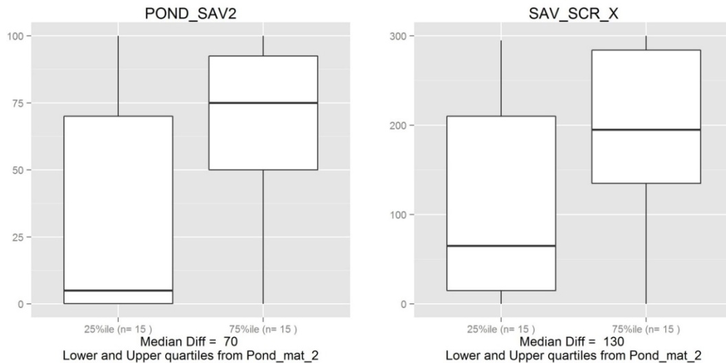
Figure A2-20. Responses of surface mats to SAV cover and index scores (units: cover of pond surface, and dimensionless index score).
