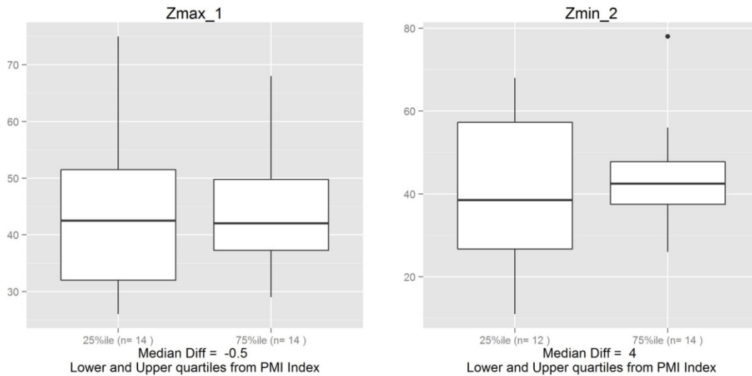
Figure A2-21. Response of macroinvertebrates to water depths (units: cm).
