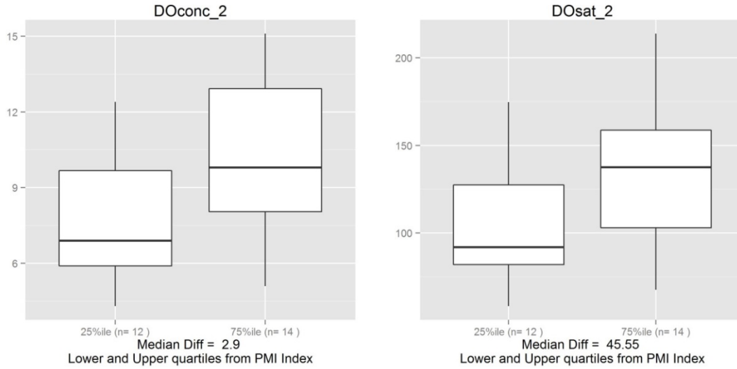
Figure A2-23. Response of macroinvertebrates to DO concentrations (units: mg/L and % saturation).
