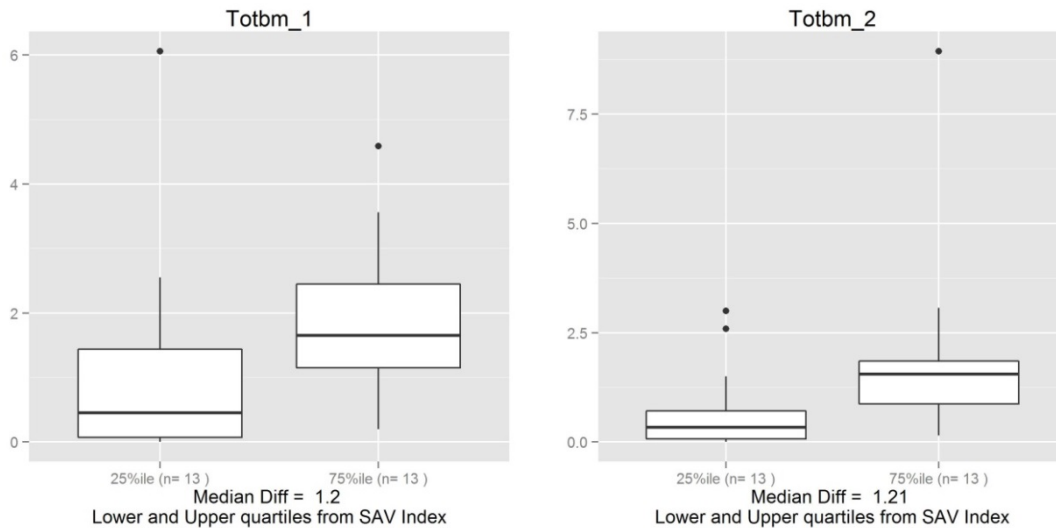
Figure A2-8. Response of SAV index to total invertebrate biomass (units g/m 2 ).
