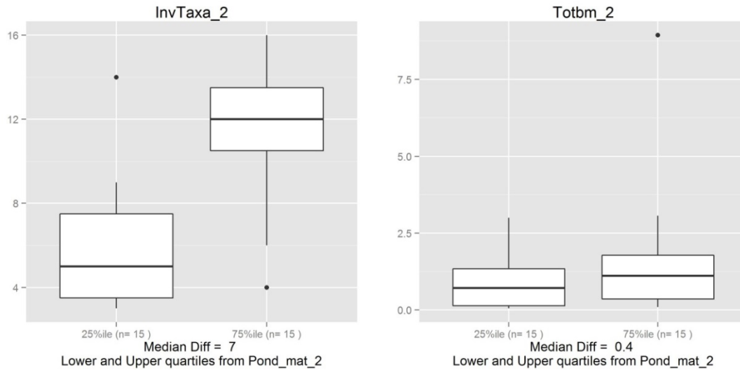
Figure A2-19. Response of surface mats to invertebrate taxa richness and total biomass (units: number of taxa and g/m 2 ).
