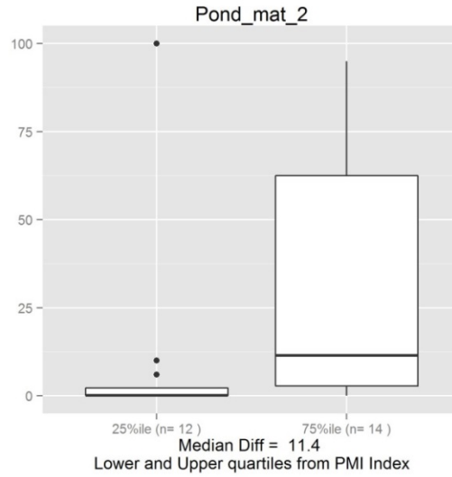
Figure A2-29. Response of macroinvertebrates to surface mat cover (units: cover of pond surface). GOOD sites also had higher cover of surface mats than POOR sites.
